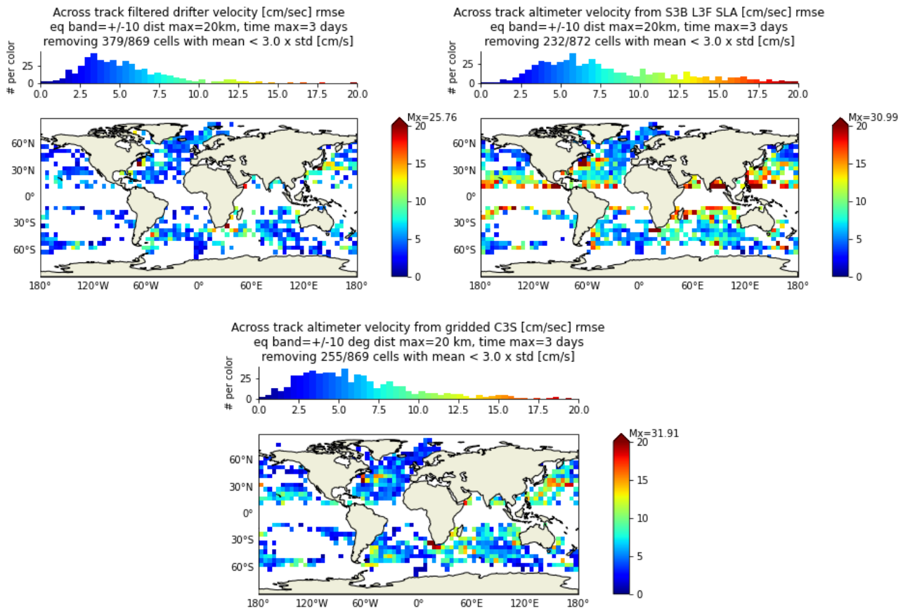
Figure 32. Results from the tri-collocation method between drifters, S3B along track altimetry, and gridded C3S across track geostrophic anomaly after removing the \pm 10 degrees equatorial band (geostrophic equation not valid), keeping matchups where distance is less or equal to 20km, time difference is less than 3 days. Only RMSE results where bootstrapping results are reliable (the variability of the result is less than the result) are plotted.
