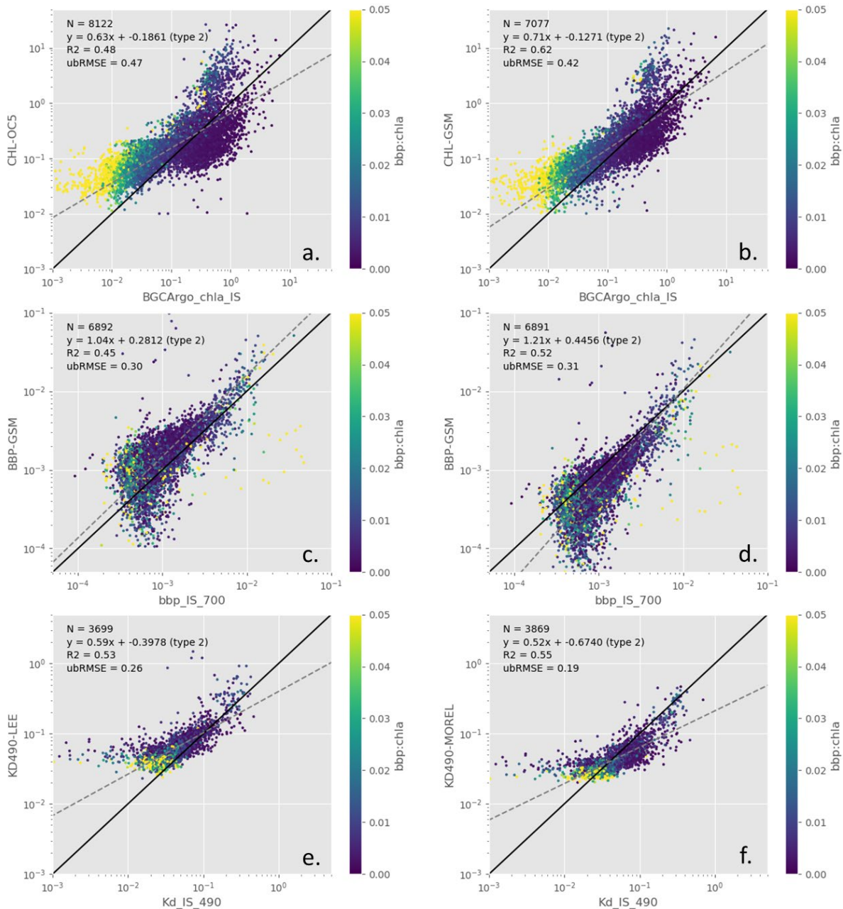
Figure 35. Scatter plot of the chlorophyll concentration (a. for OC5, b. for GSM), BBP without and with modification of the wavelength (c., d.) and Kd (e. for Lee, f. for Morel) derived from ocean colour against the in situ measurements from BGC-Argo floats. The colour of the dot corresponds to the ratio BBP/CHL estimated from BGC-Argo data. Due to the lognormal distribution of the three parameters (chl, Kd and BBp), the validation plots are given on a logscale.
