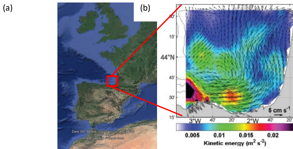
Figure 11. (a) Location of the study area. (b) Surface currents and kinetic energy per unit of mass (in m^2 \cdot s^{-2} ) for winter from HF radar observations (Caballero et al., 2020).
