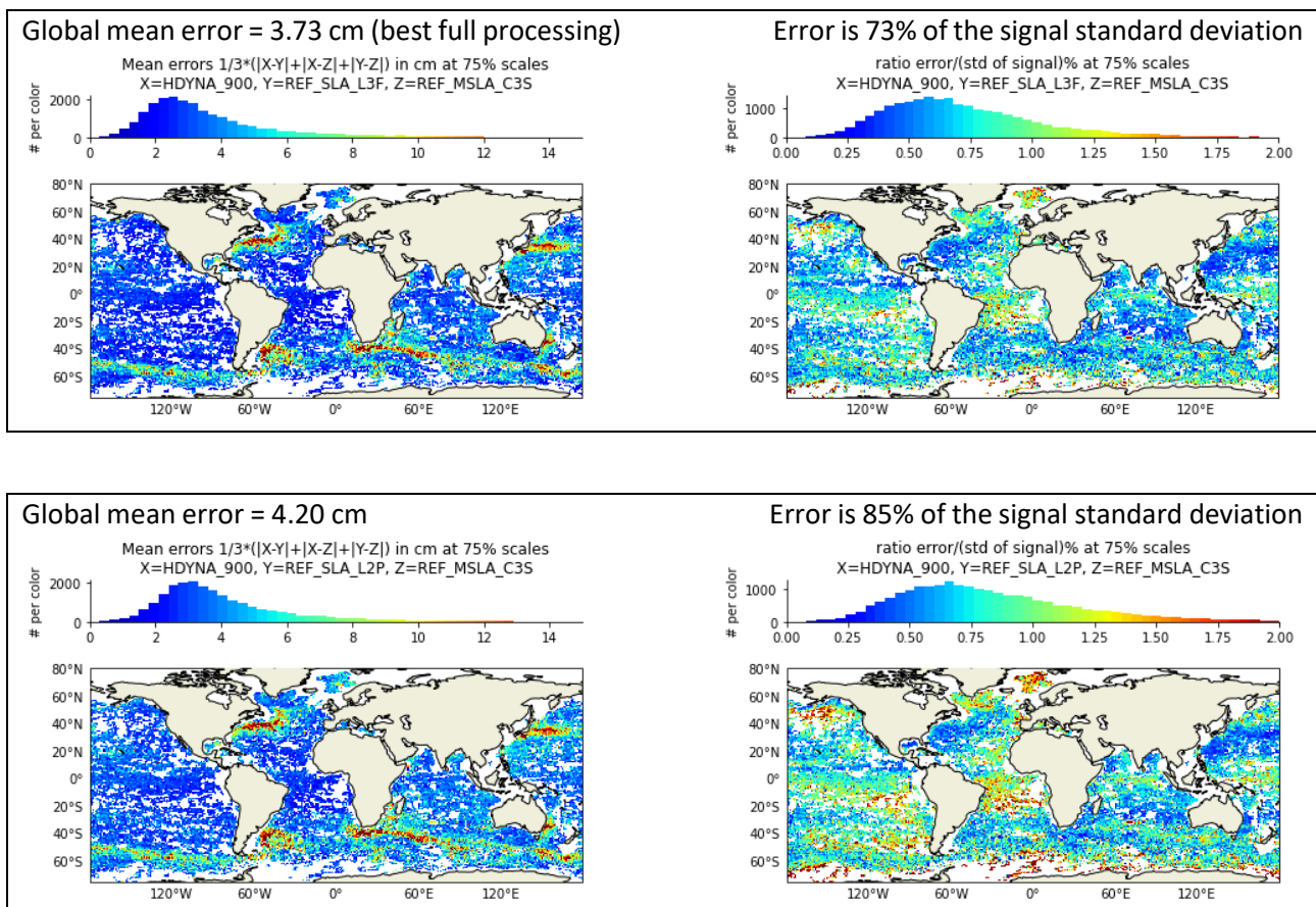
Figure 20. Mean error from the combination of 3 dataset: Dynamic height anomalies, gridded combined C3S sea level anomalies, and different along-track sea level anomalies: top) L3F best, bot) L2P least corrected.
